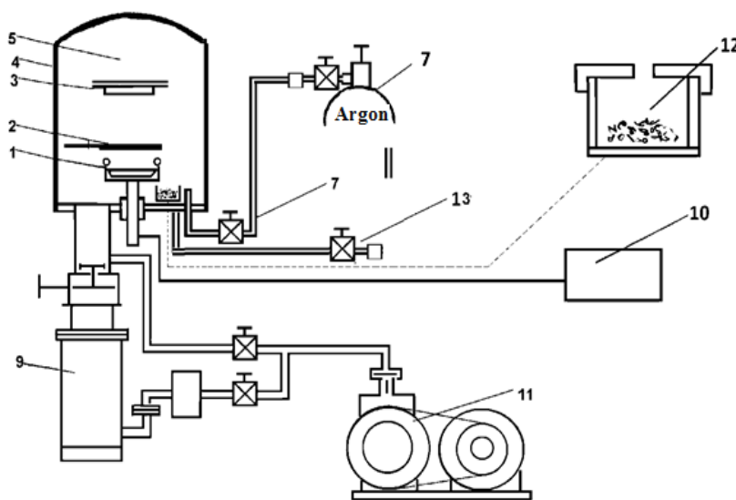
1 – graphite target, 2 – damper, 3 – a sample holder (substrate), 4 – duralumin stand chair, 5 – the working vacuum chamber, 6 – leak valve, 7 – and argon balloon, 8 – cylinder gases (for conventional methods of methane gas), 9 – diffusion pump, 10 – high-voltage power supply, 11 – backing pump, 12 – case for the sublime substances, 13 – capacity for liquid aromatics
